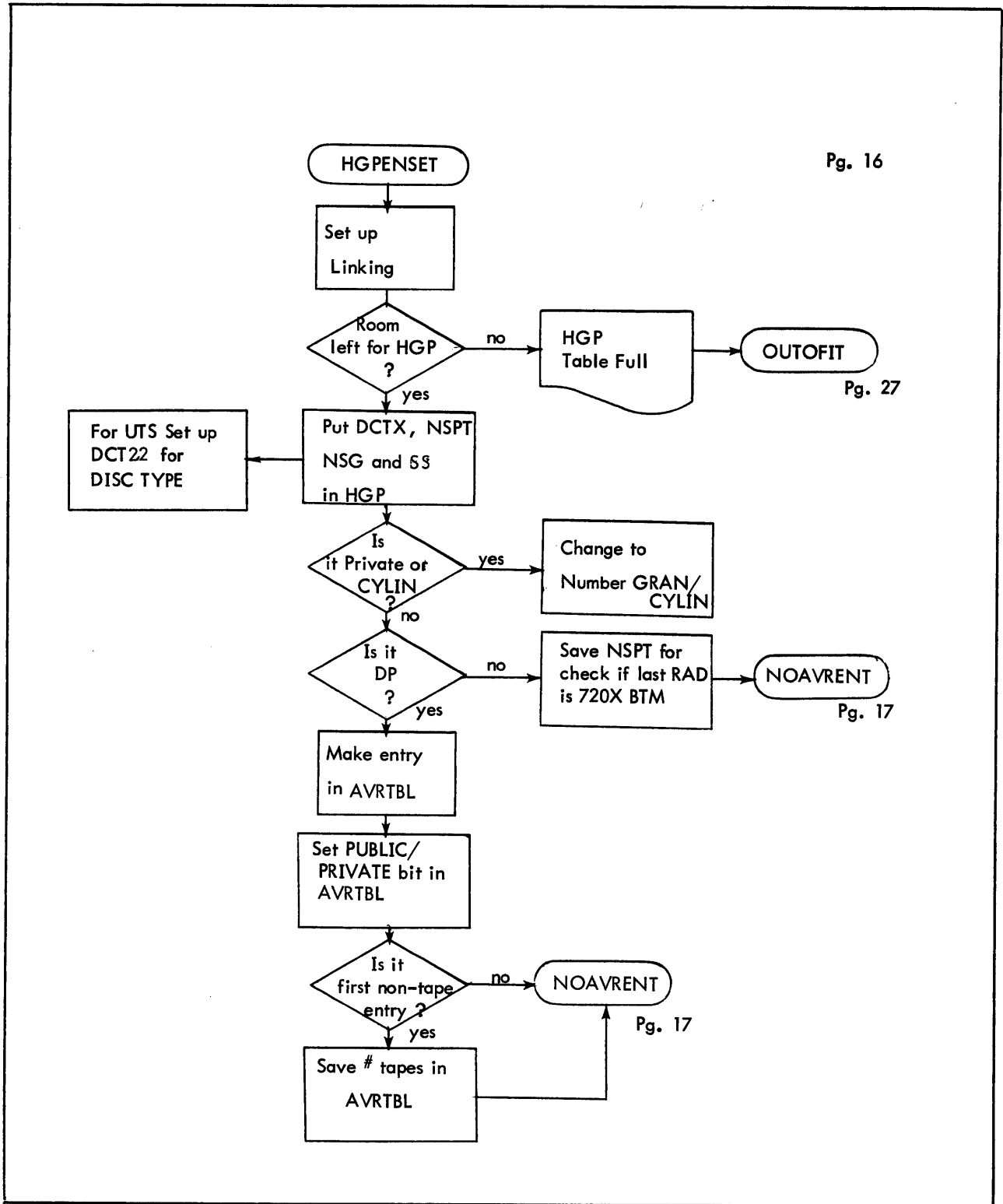
Figure 2-9. Flow Diagram of UBCHAN (Cont.)
