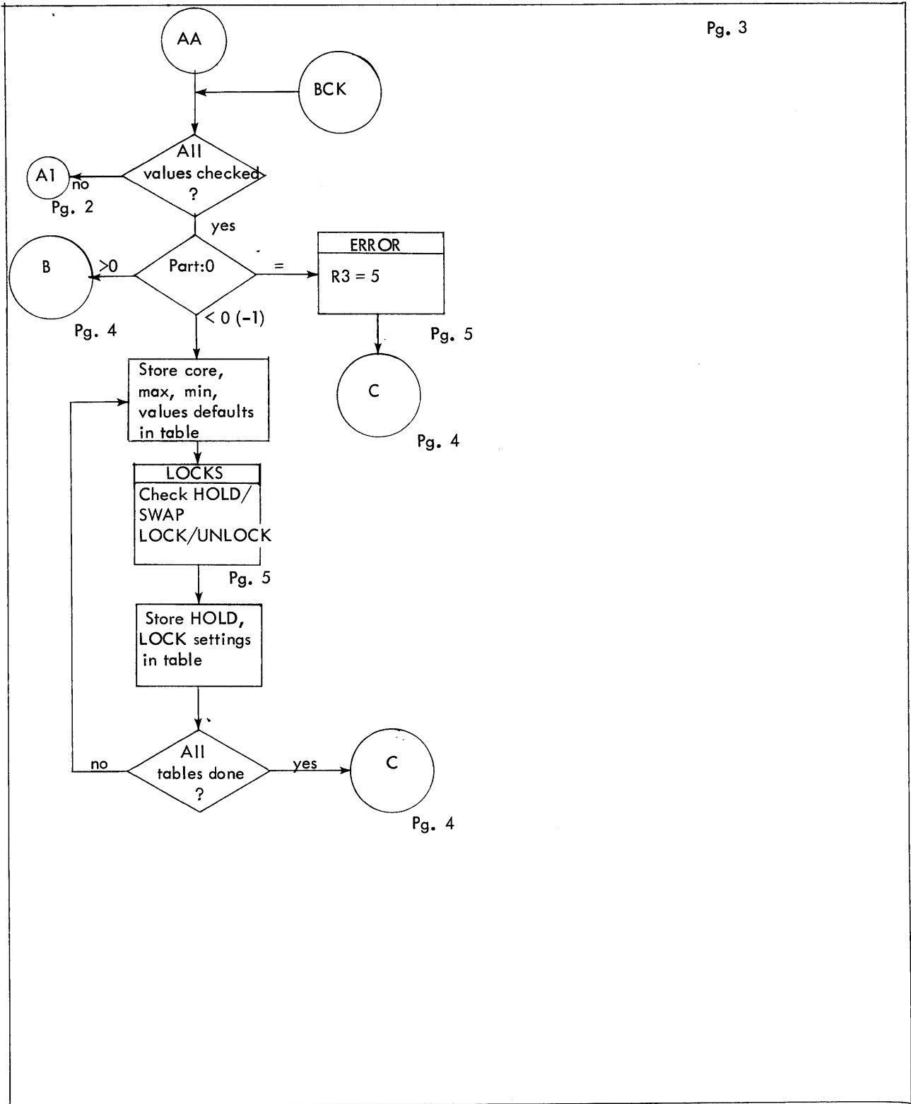
Figure 2-20. Flow Diagram of XPART (Cont.)
