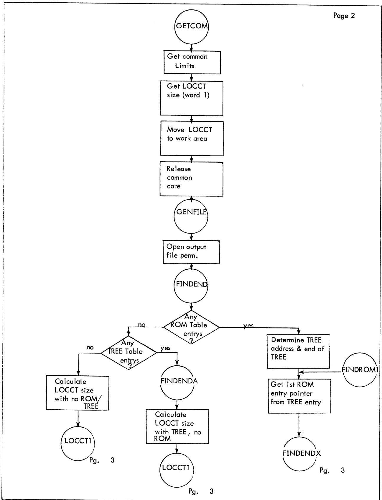
Figure 5-2. Flow Diagram of LOCCT (Cont.)
