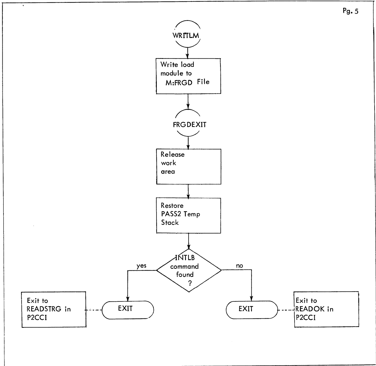
Figure 2-19. Flow Diagram of FRGD (Cont.)
