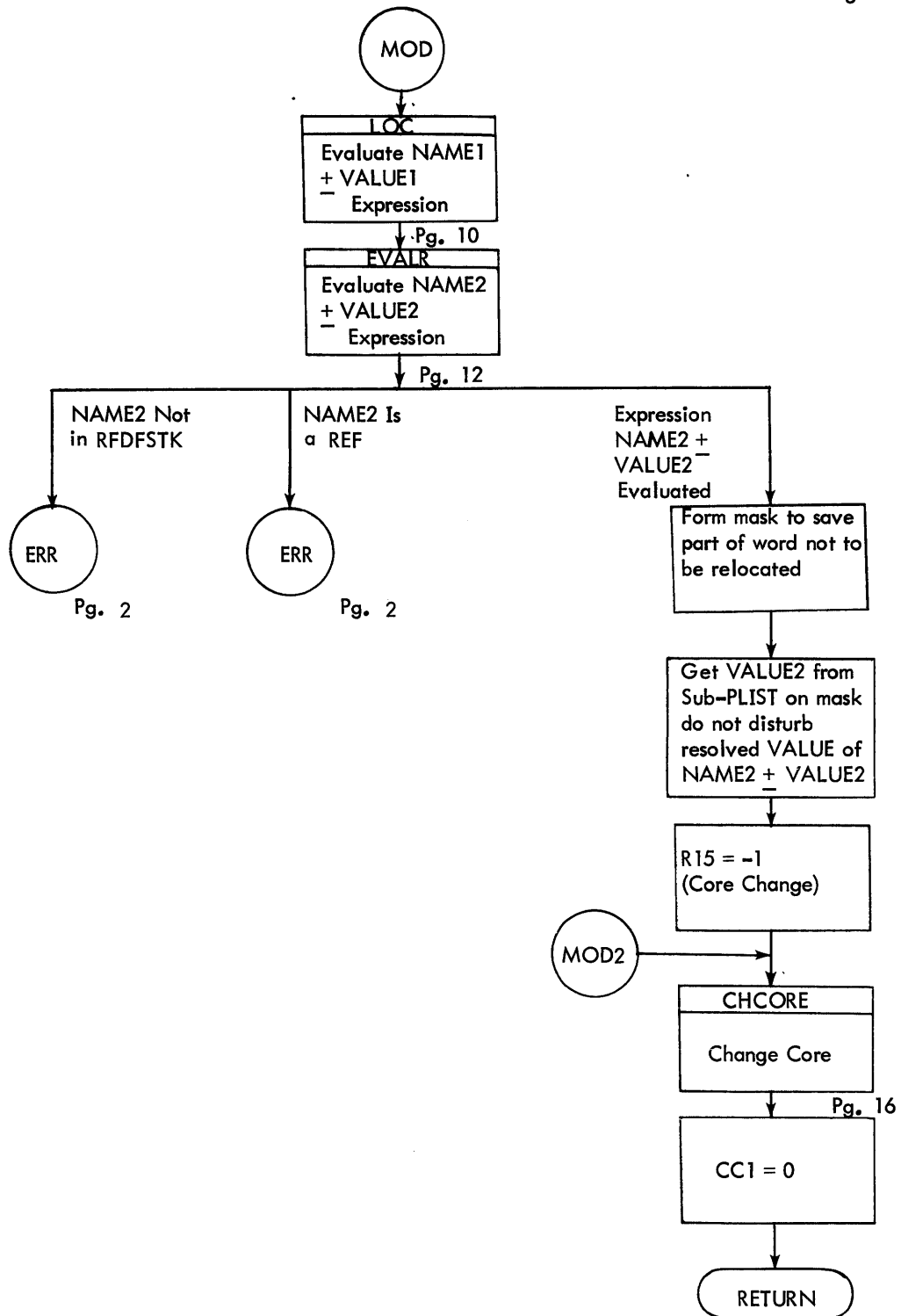
Figure 6-15. Flow Diagram of MODIFY (Cont.) (Process MOD SubPLIST)
