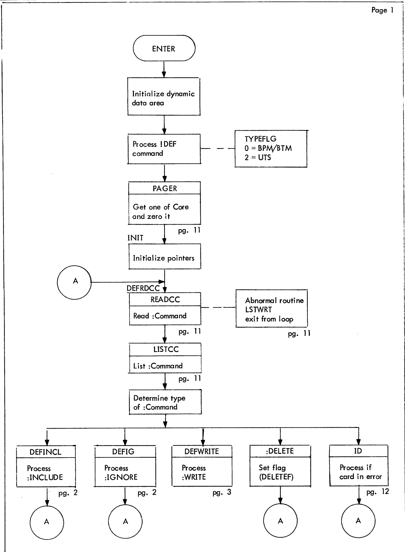
Figure C-1. Flow Diagram of DEF
