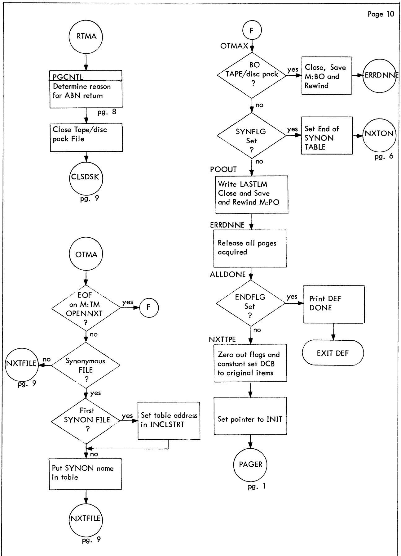
Figure C-1. Flow Diagram of DEF (Cont.)
