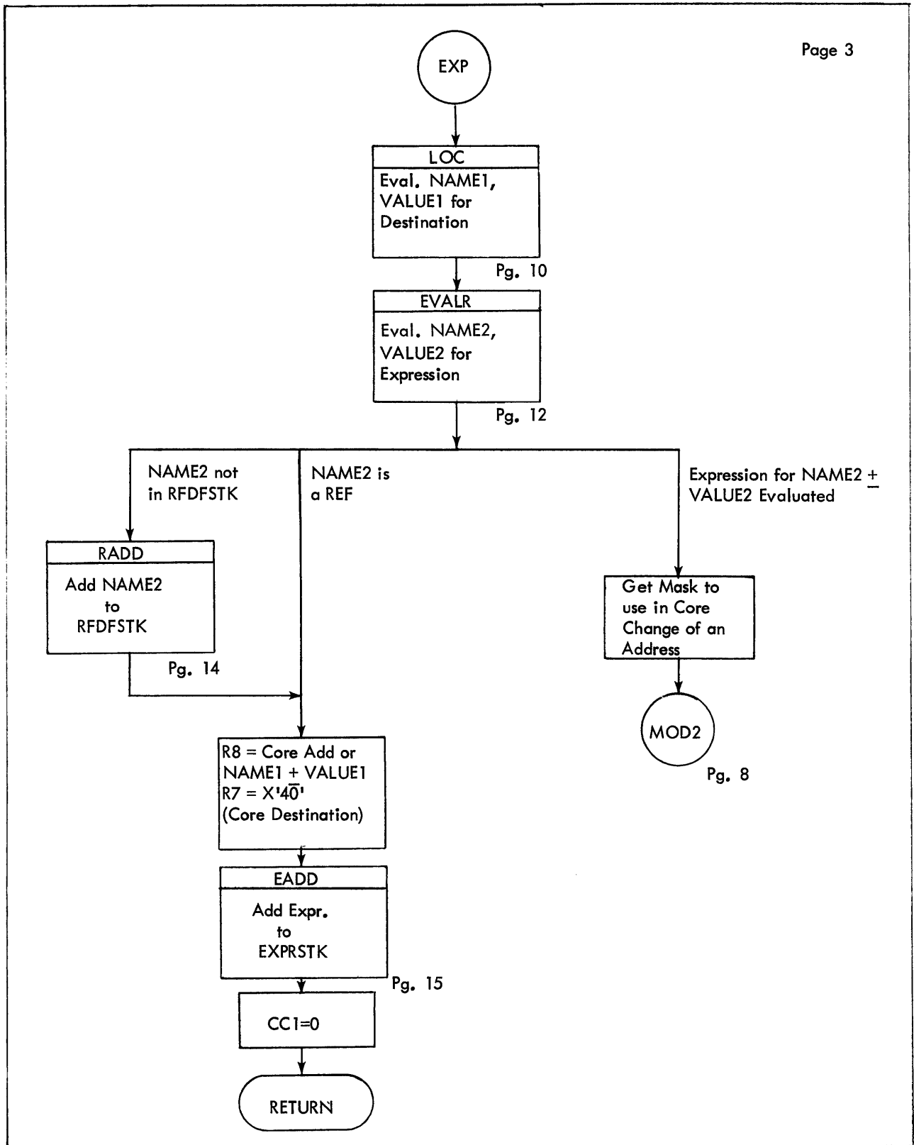
Figure 6-15. Flow Diagram of MODIFY (Cont.) (Process EXPR SubPLIST)
