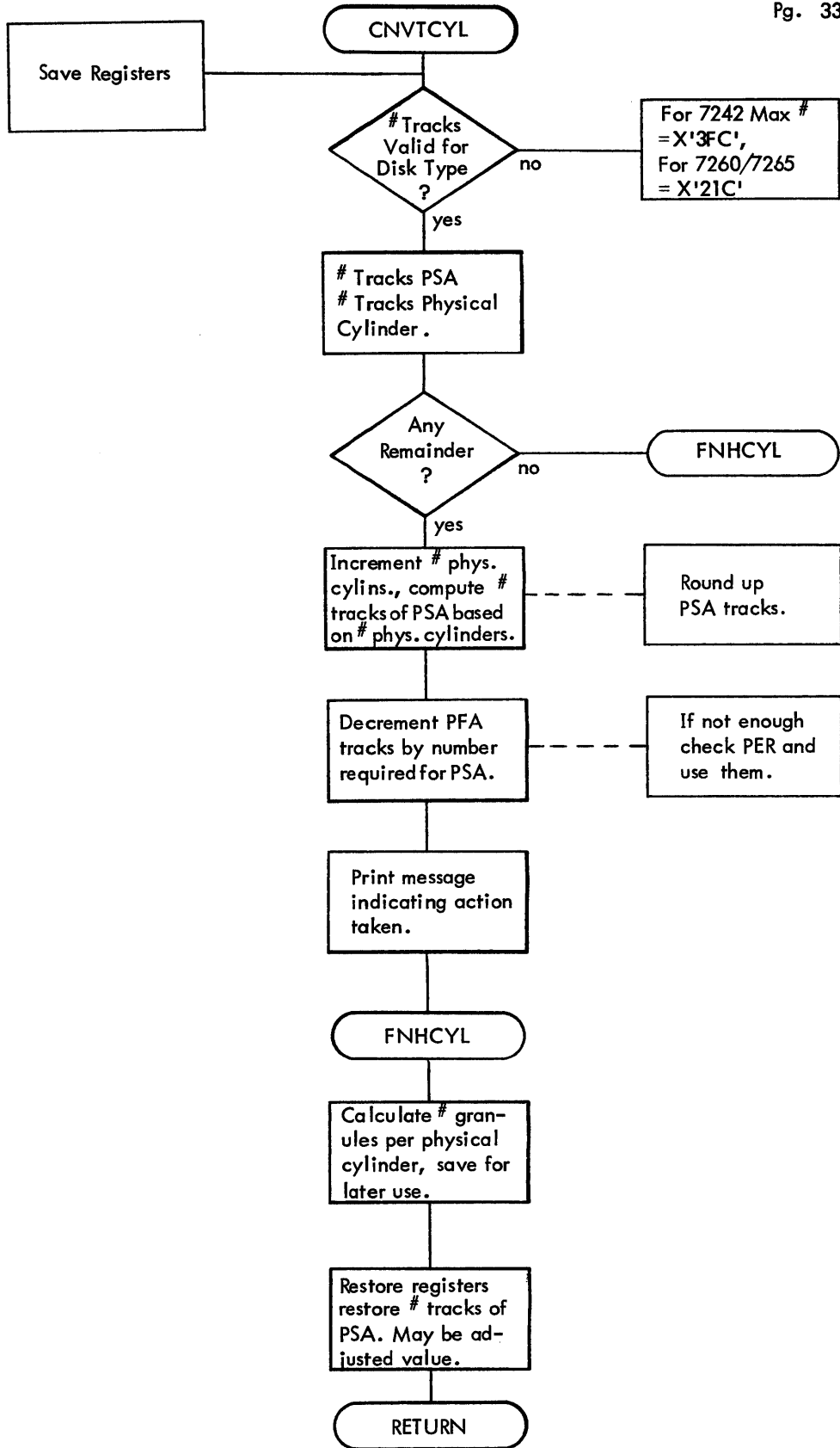
Figure 2-9. Flow Diagram of UBCHAN (cont.)
