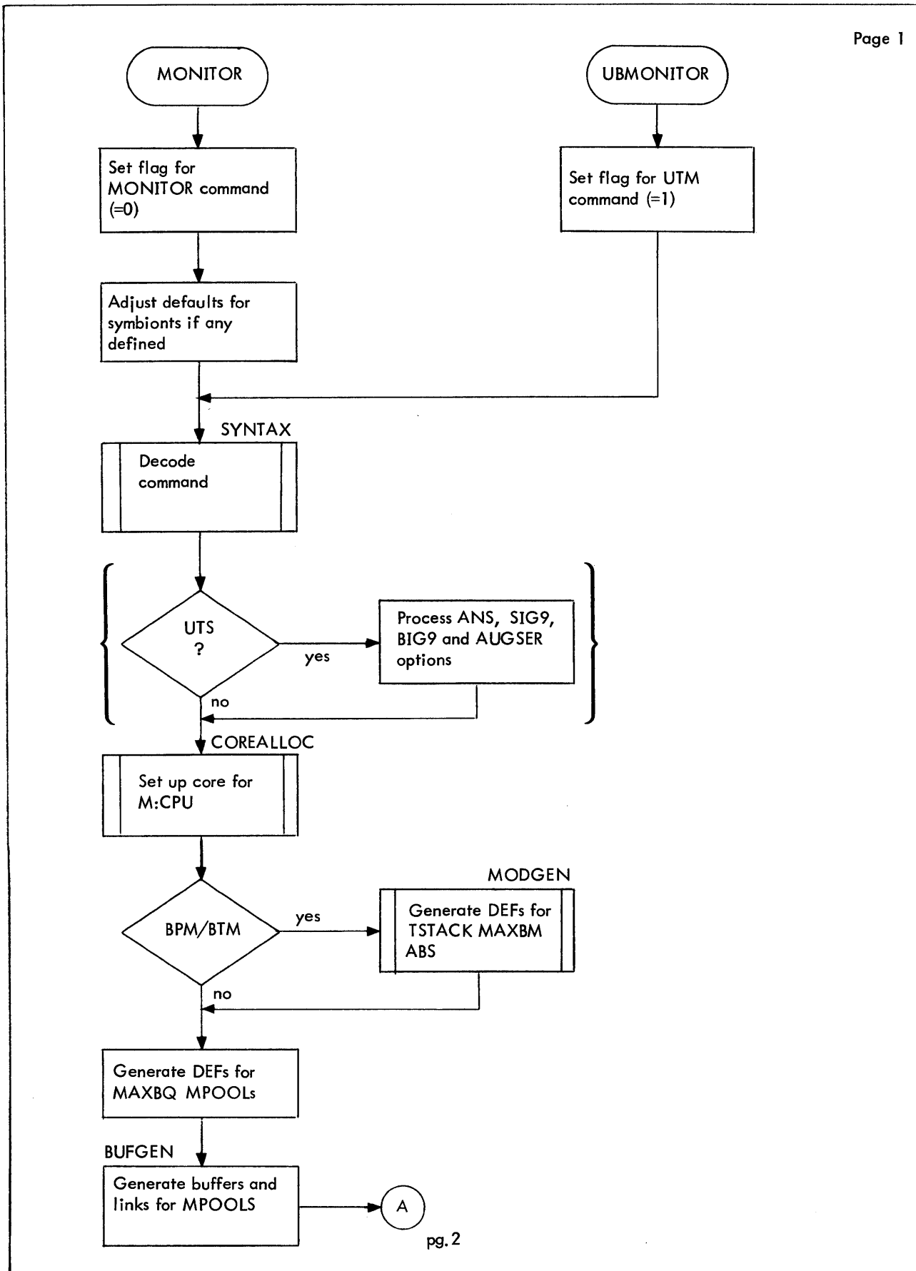
Figure 2-11. Flow Diagram of XMONITOR
