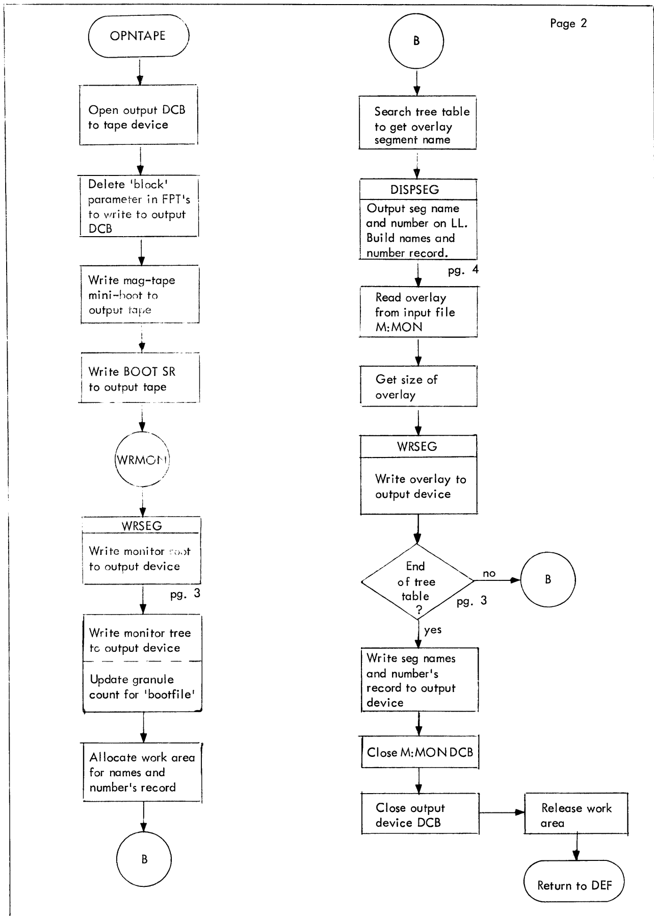
Figure A-1. Flow Diagram of BPMBT (Cont.)
