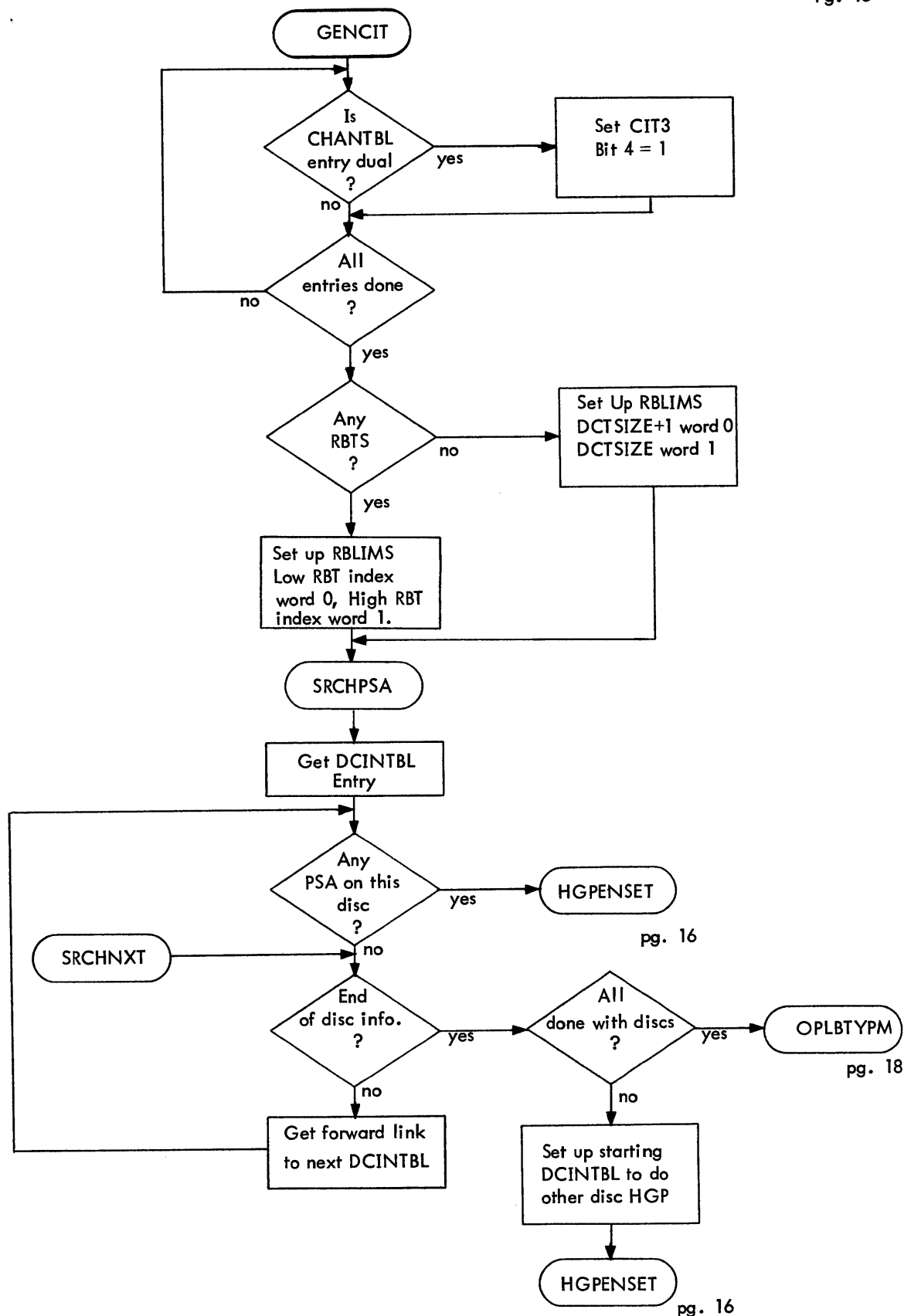
Figure 2-9. Flow Diagram of UBCCHAN (cont.)
