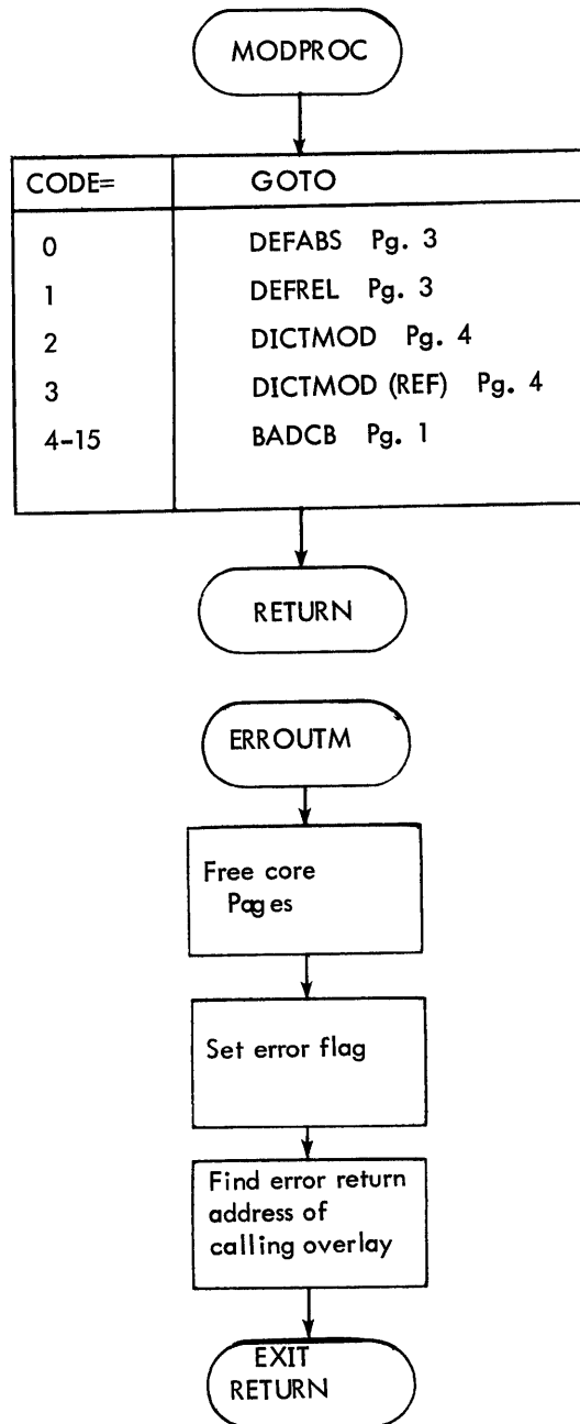
Figure 6-27 Flow Diagram of MODGEN (Cont.)
