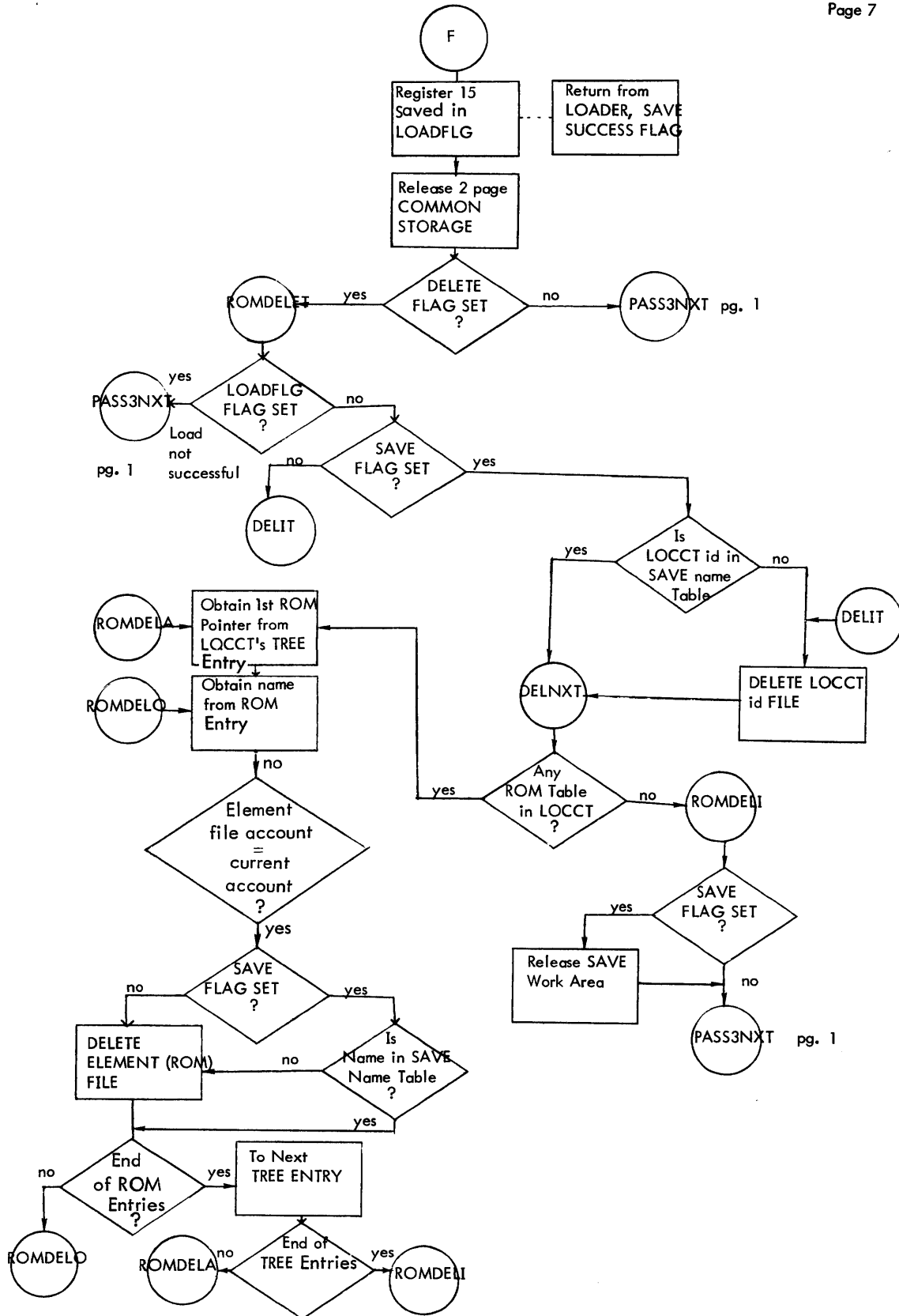
Figure 3-1. Flow Diagram of PASS3 (CONT)
