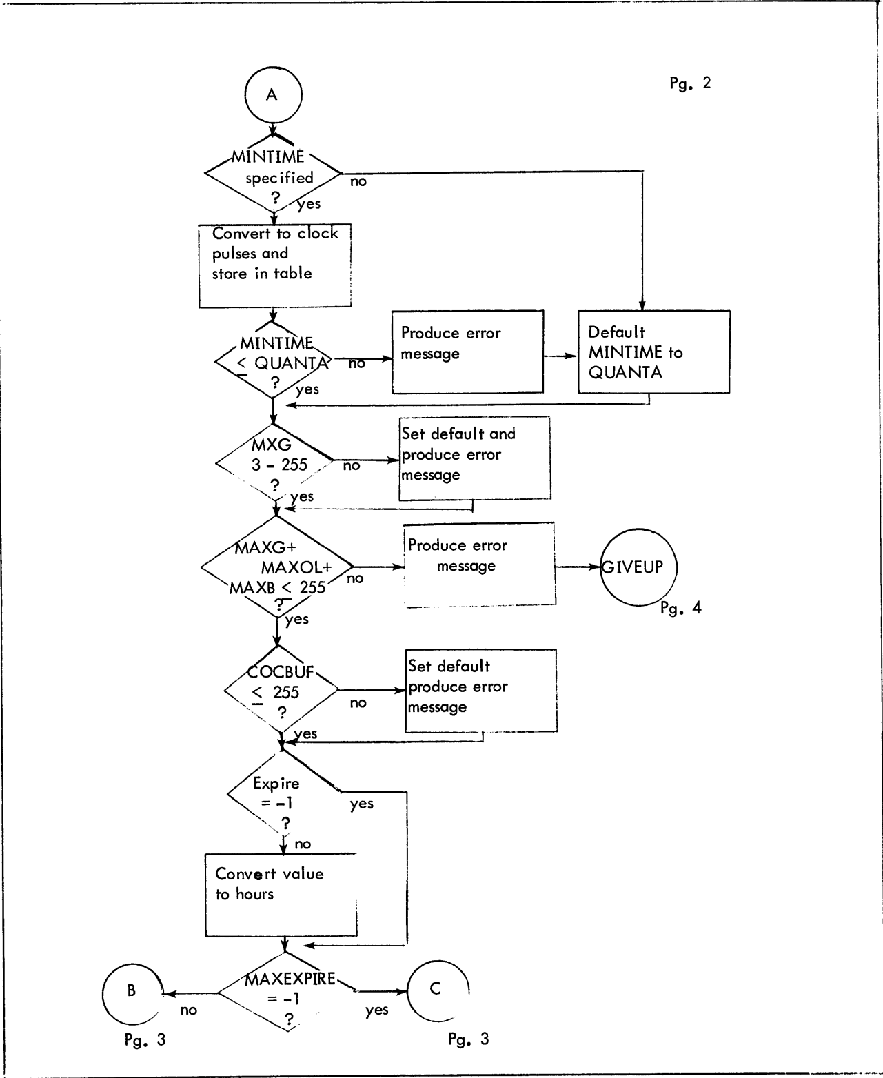
Figure 2-16. Flow Diagram of IMC (Cont.)
