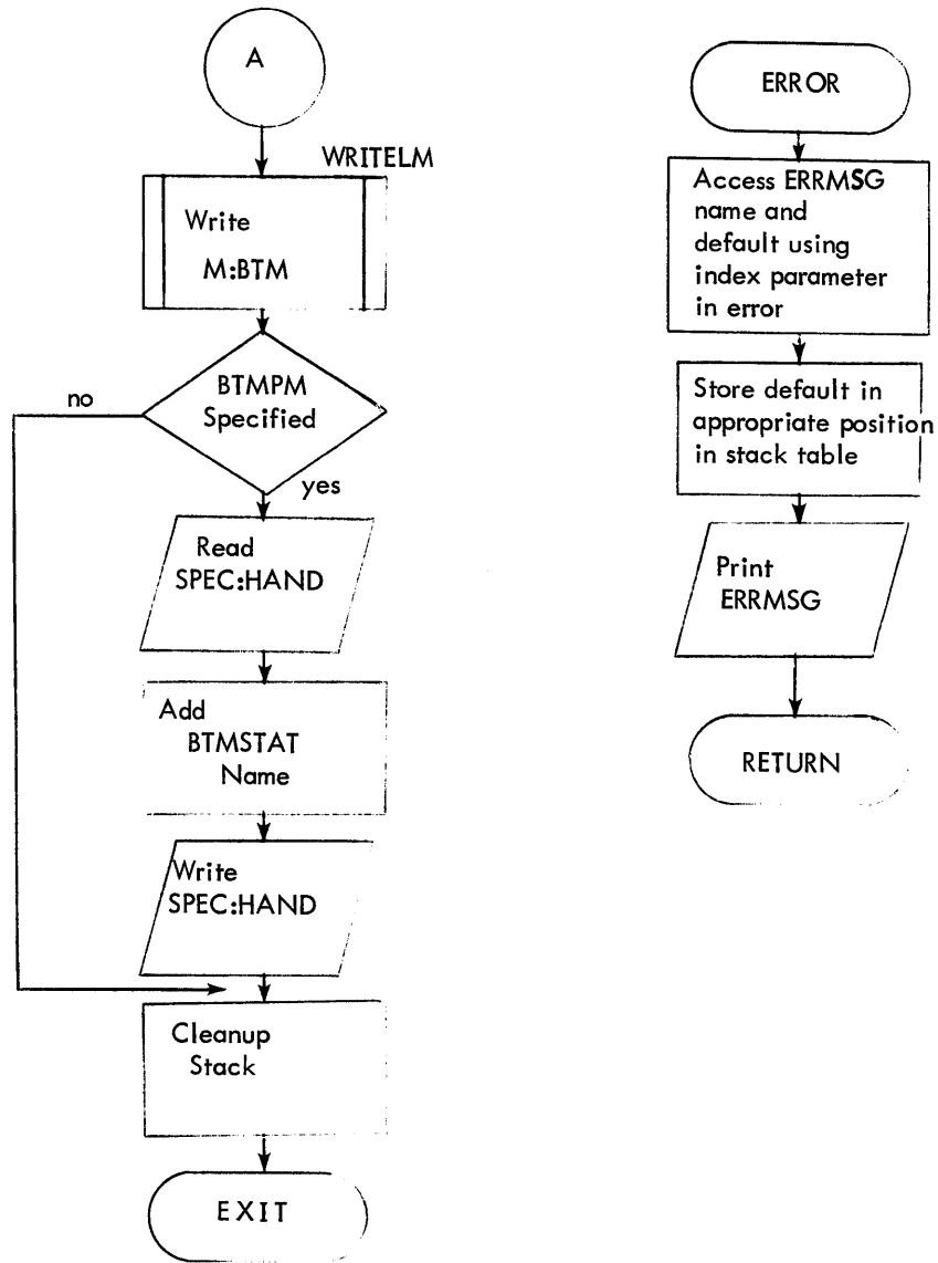
Figure 2-14. Flow Diagram of BTM (Cont.)
