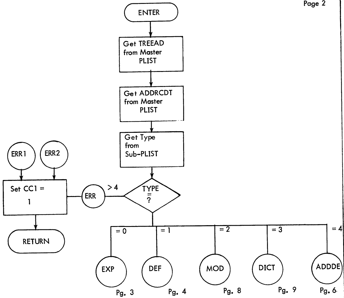
Figure 6-15. Flow Diagram of MODIFY (Cont.) (Entry Point)
