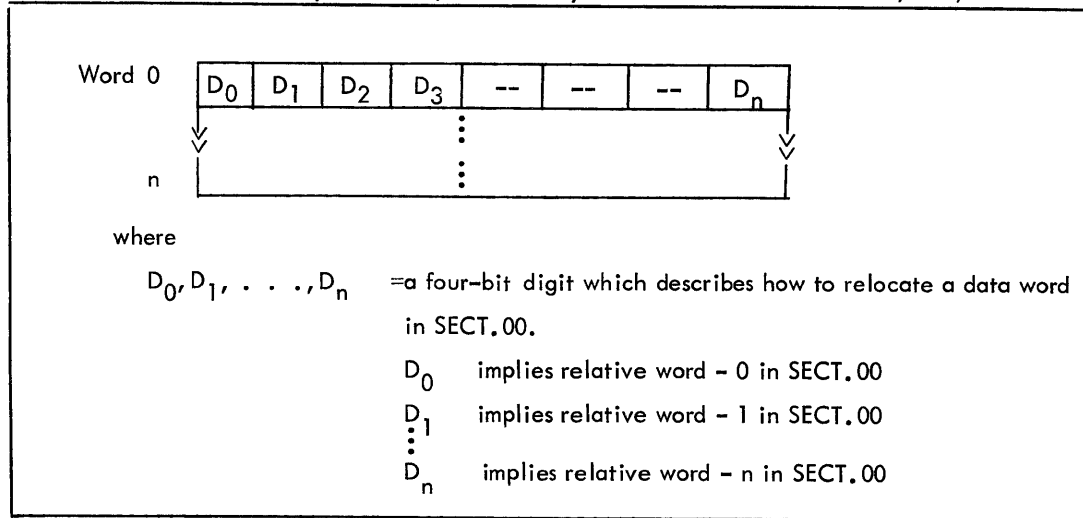
Figure 6-8 RELDICT Format
