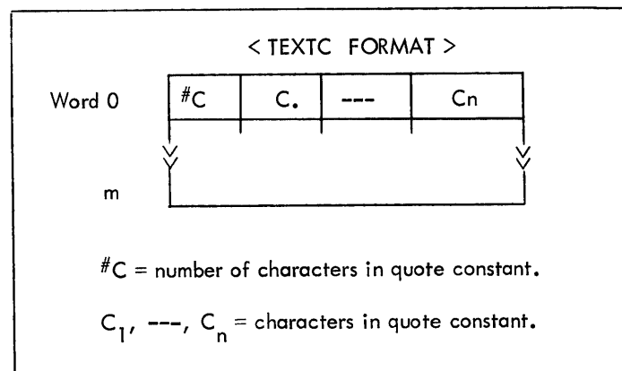
Figure 6-21. Quote Constant
