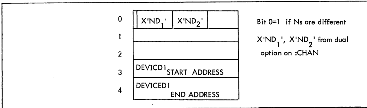
Figure 2-2. CHANTBL Entry
