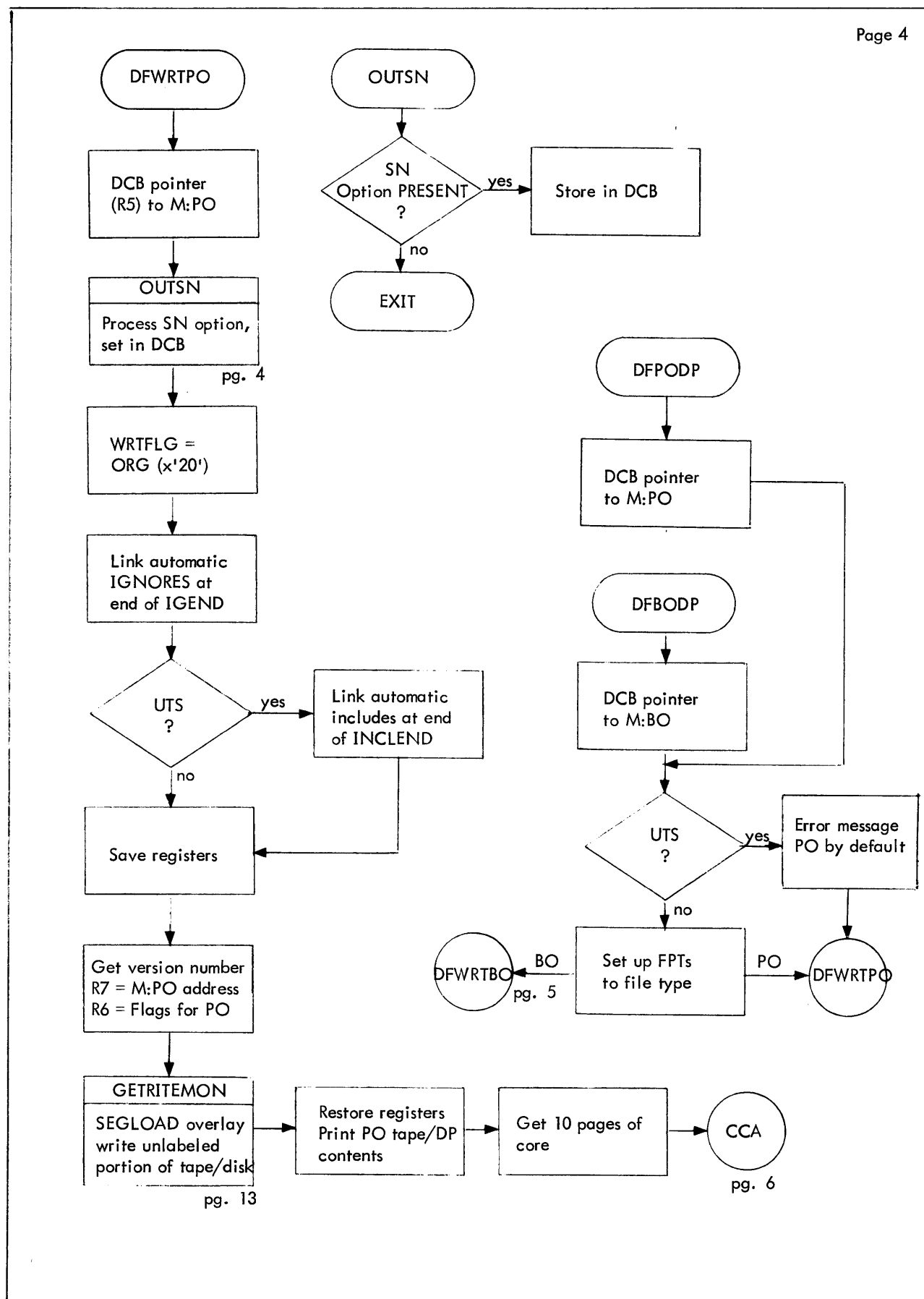
Figure C-1. Flow Diagram of DEF (Cont.)
