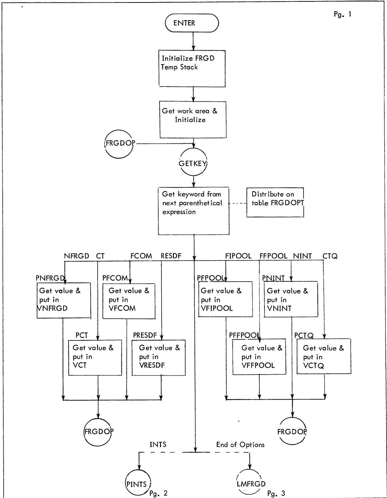
Figure 2-19. Flow Diagram of FRGD
