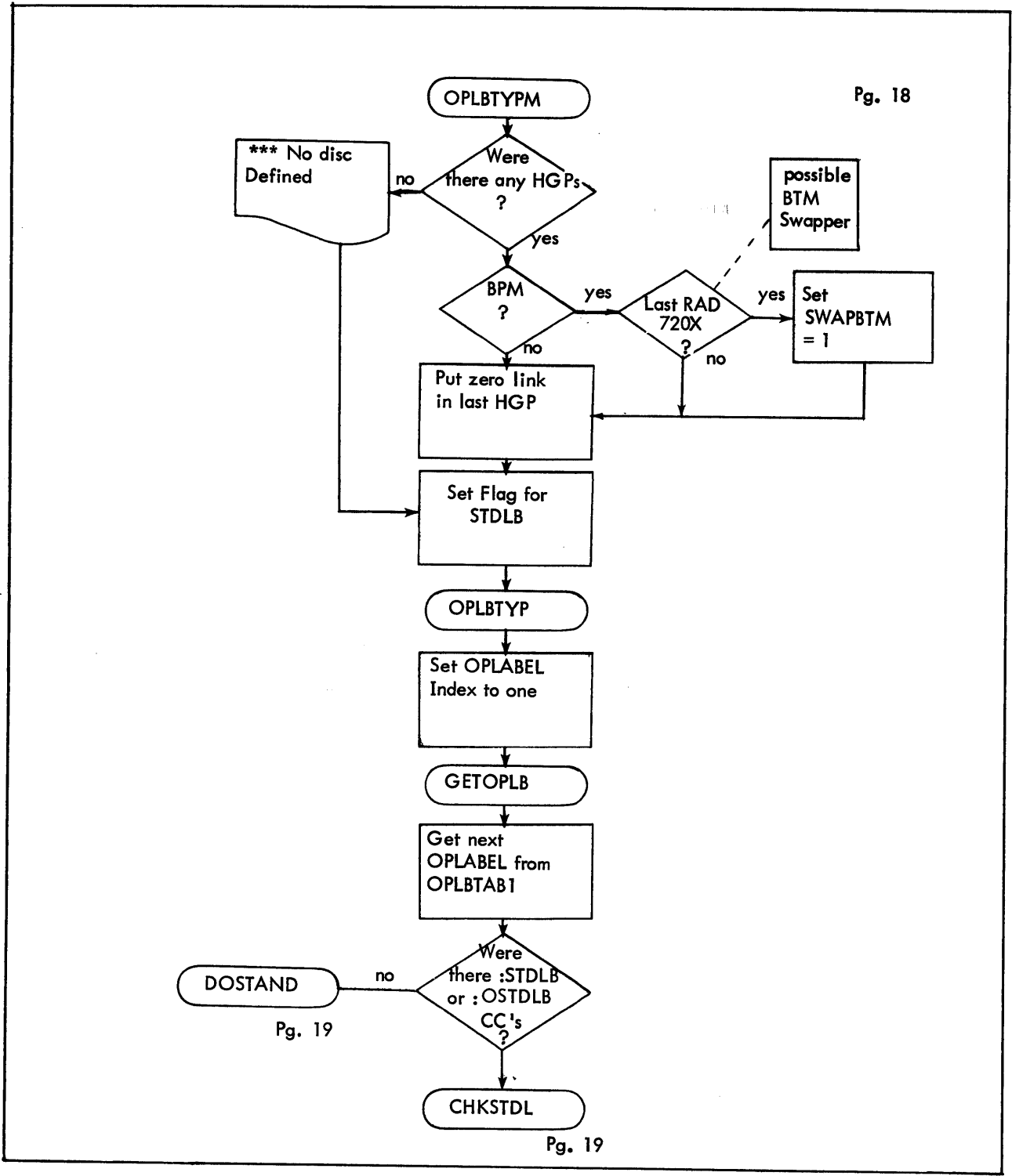
Figure 2-9. Flow Diagram of UBCCHAN (Cont.)
