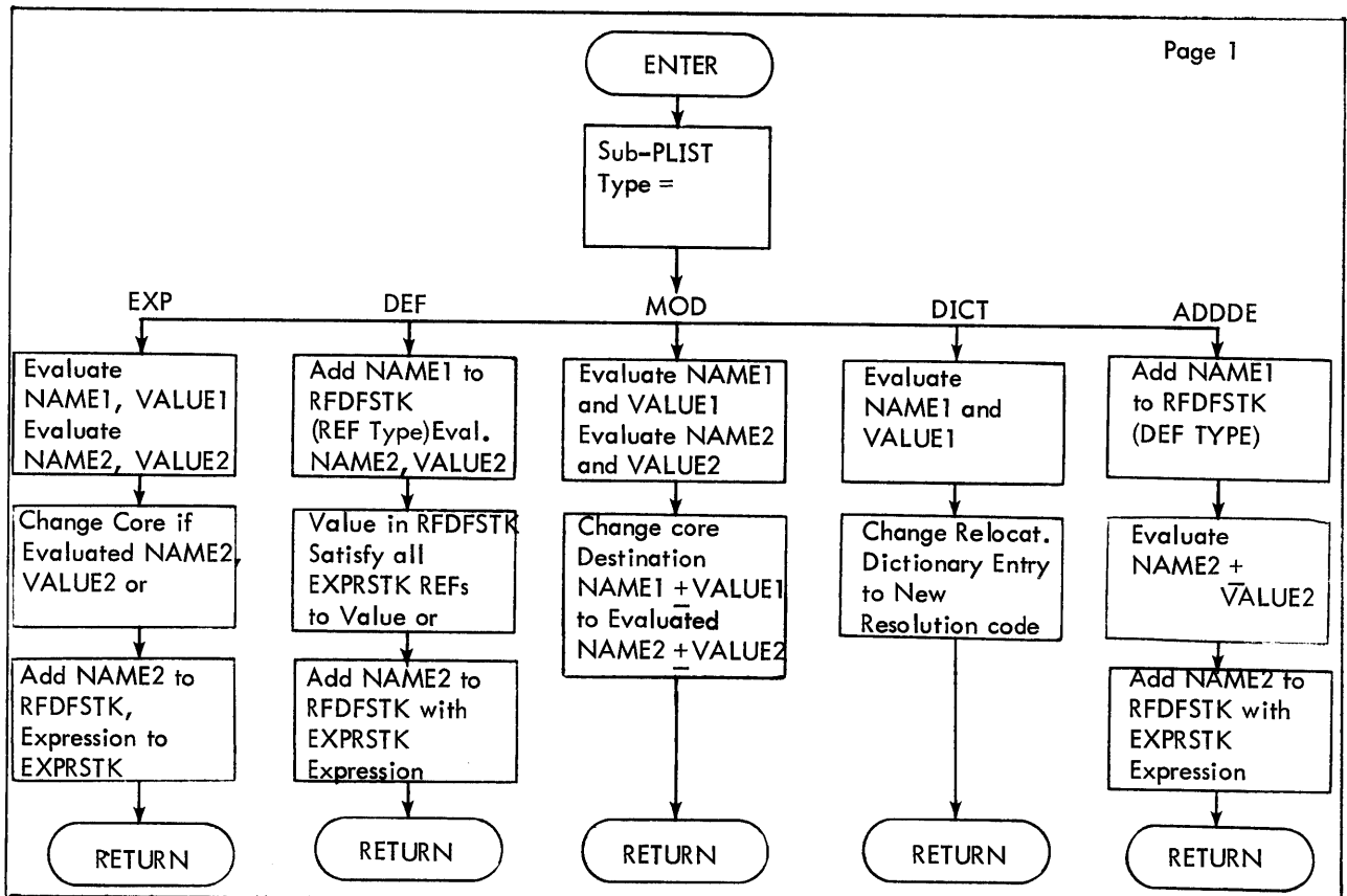
Figure 6-15. Flow Diagram of MODIFY (General Flow)
