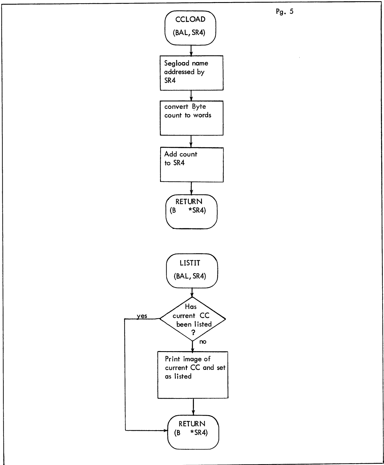
Figure 2-1 Flow Diagram of P2CCI (Cont.)
