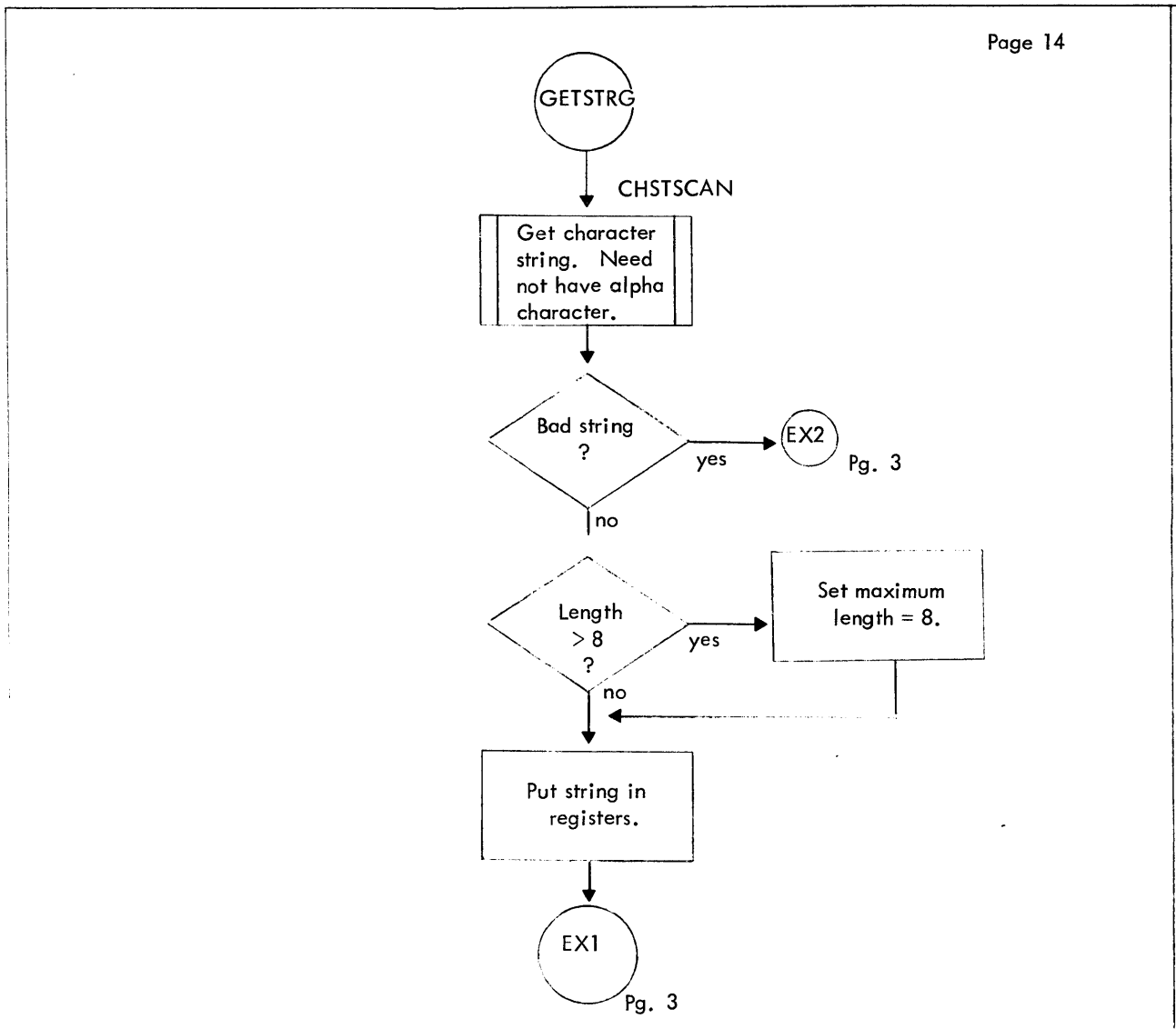
Figure 6-26. Flow Diagram of SYNTAX (Cont.)
