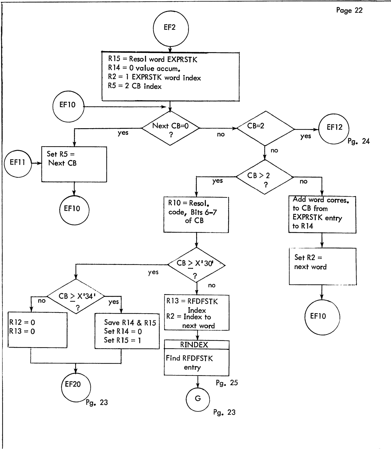
Figure 6-15. Flow Diagram of MODIFY (Cont.) ( Subroutines )
