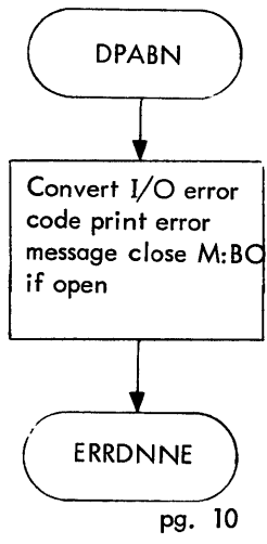
Figure C-1. Flow Diagram of DEF (Cont.)
