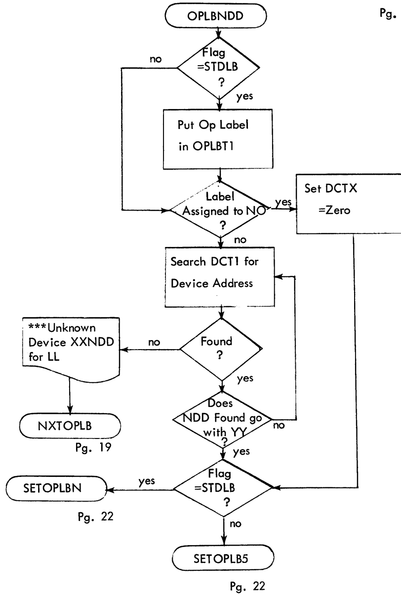
Figure 2-9. Flow Diagram of UBCHAN (Cont.)
