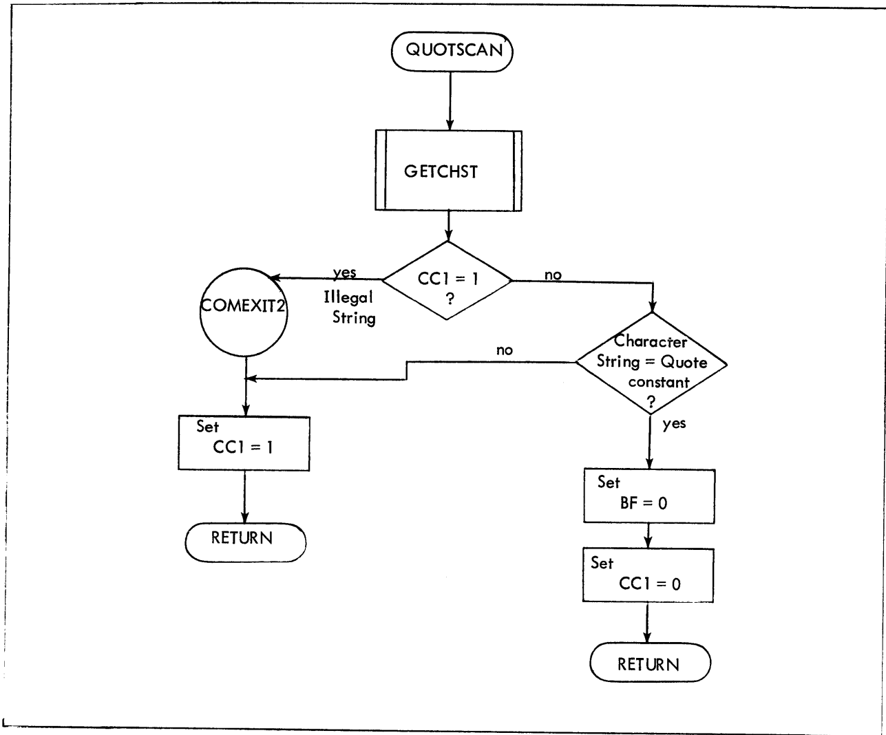
Figure 6-22. Flow Diagram of QUOTSCAN
