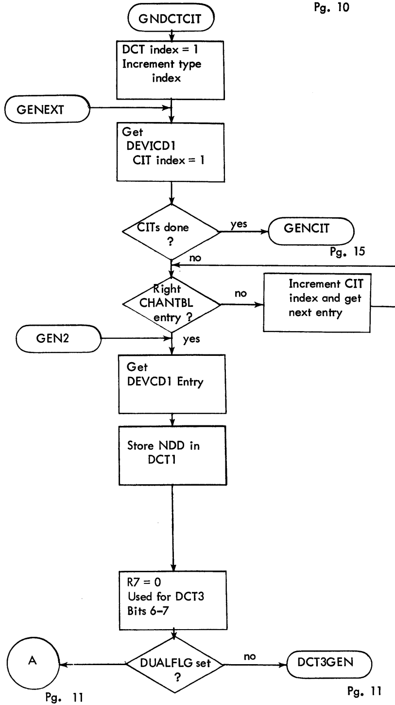
Figure 2-9. Flow Diagram of UBCCHAN (Cont.)
