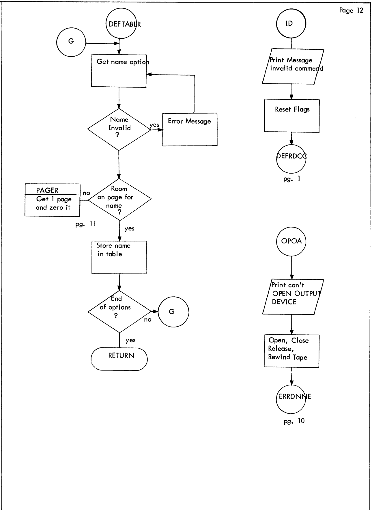
Figure 4-1. Flow Diagram of DEF (CONT)
