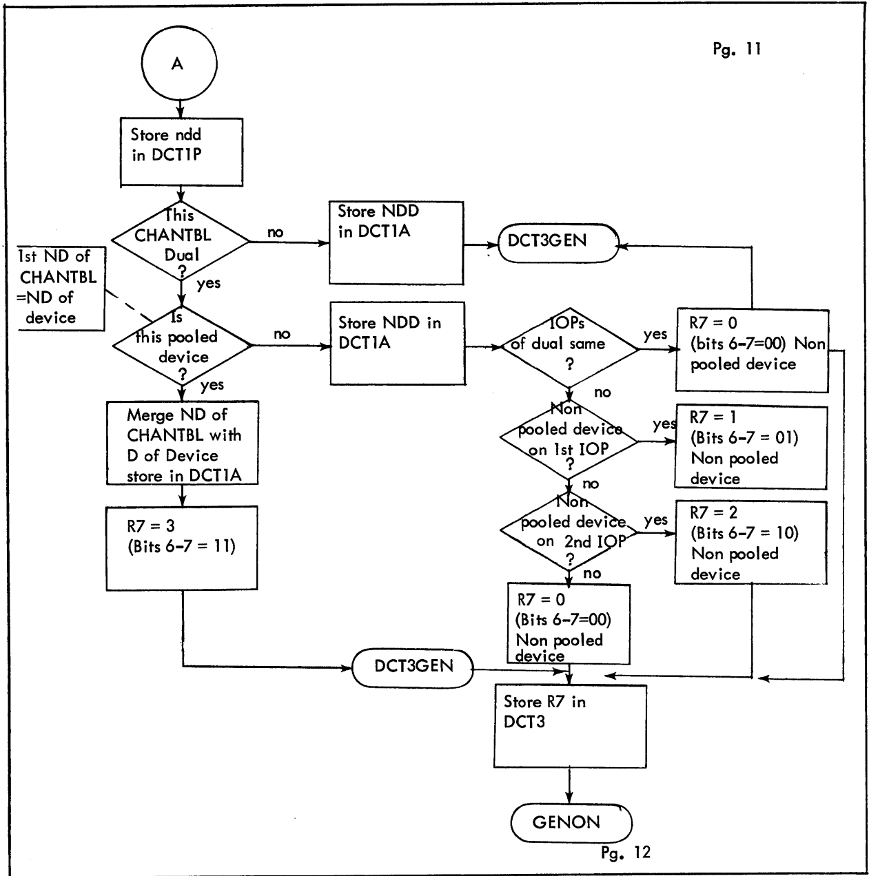
Figure 2-9. Flow Diagram of UBCCHAN (Cont.)
