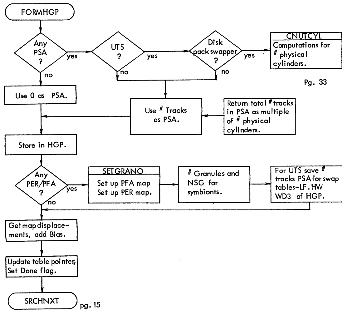
Figure 2-9. Flow Diagram of UBCHAN (cont.)
