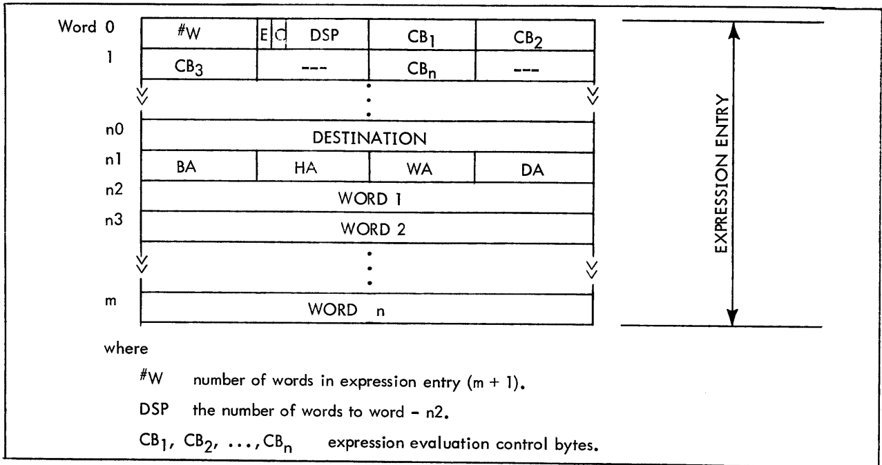
Figure 6-7 EXPRSTK Format
