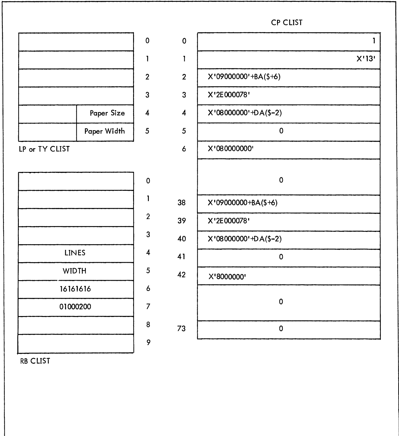
Figure 2-7. Special CLISTS
